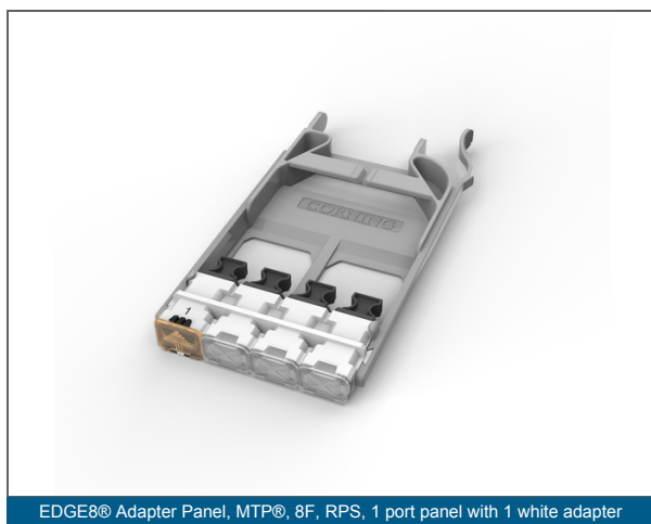
EDGE8® Adapter Panel, MTP®, 8F, RPS, 1 port panel with 1 white adapter
